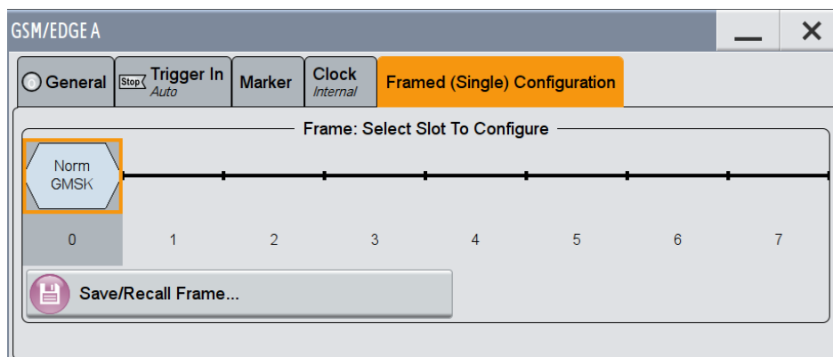
Fig. 8-5: R&S SMW200A: GSM/EDGE frame configuration settings
