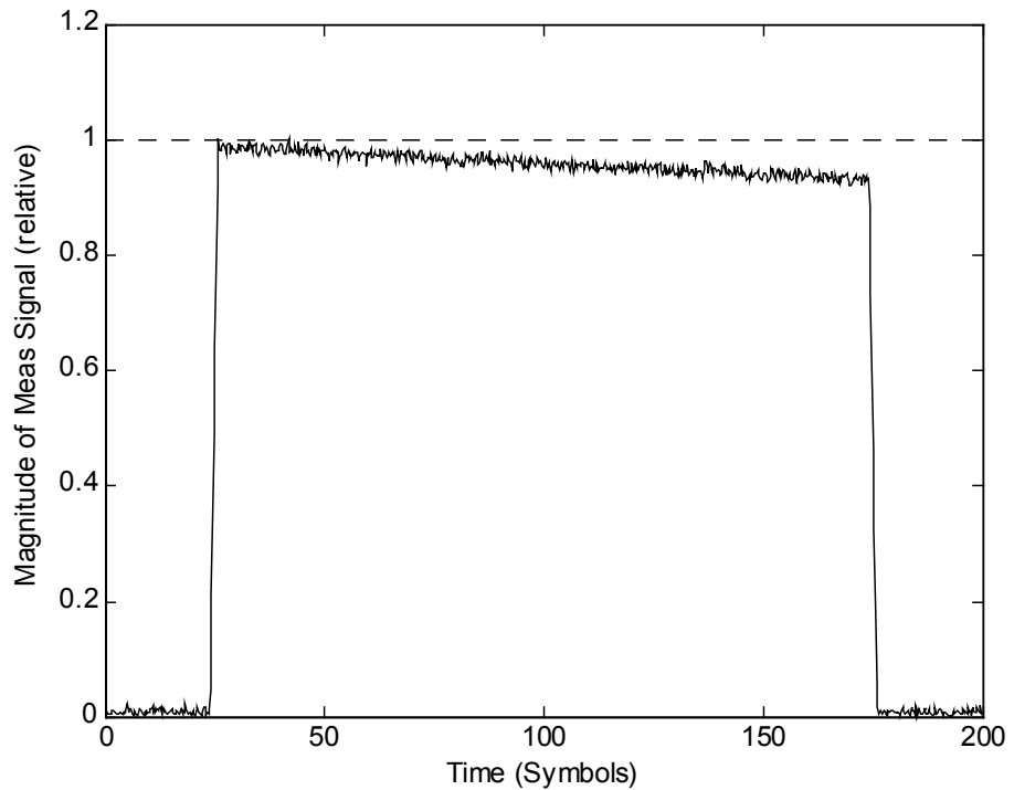
Fig. 4-56: Effect of amplitude droop
