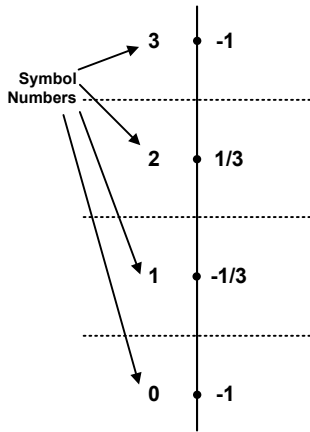
Fig. 4-23: Constellation diagram for 4FSK (NATURAL) including the logical symbol mapping
