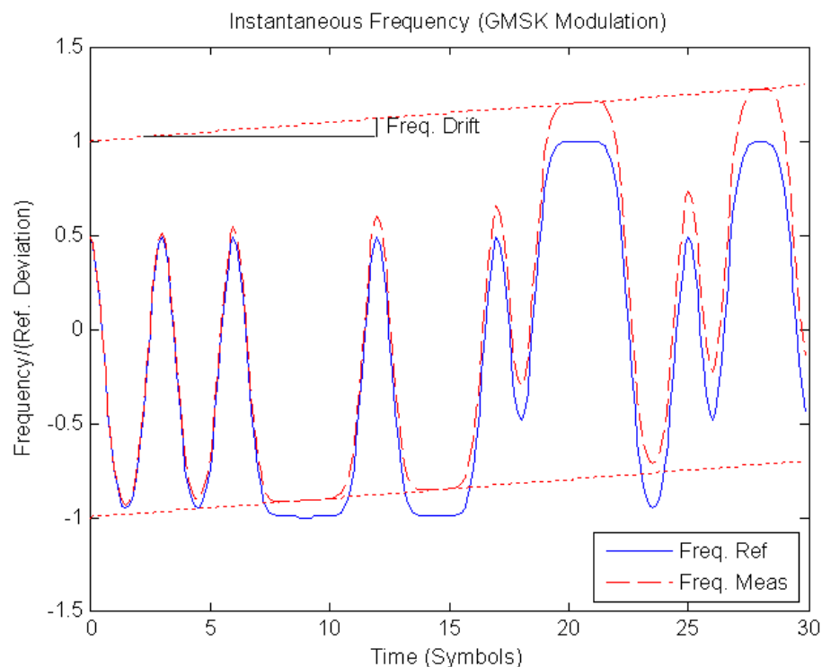
Fig. 4-60: The reference and distorted instantaneous frequency of a GMSK signal with a carrier frequency drift
