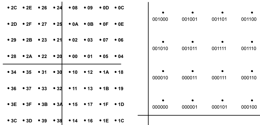
Fig. 4-33: Constellation diagram for 64QAM including the logical symbol mapping for DVB-C (hexadecimal and binary); the binary form shows the upper right section of the diagram only.
