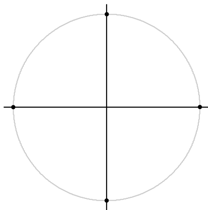
Fig. 4-20: Constellation diagram for \pi/4 DQPSK including the symbol mapping for APCO25 Phase 2, NADC, NATURAL, PDC, PHS, TETRA and TETS; the \pi/4 rotation is already compensated for
