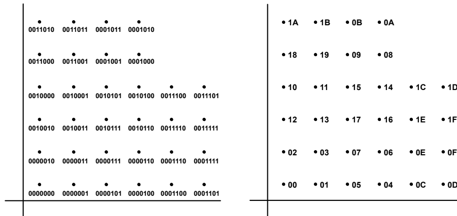
Fig. 4-34: Constellation diagram for 128QAM including the logical symbol mapping (hexadecimal and binary); the figure shows the upper right sections of the diagram only
