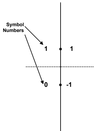
Fig. 4-22: Constellation diagram for 2FSK (NATURAL) including the logical symbol mapping
