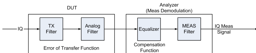
Fig. 4-47: Compensation of the transfer function's error by inserting an equalizer in the receive path
