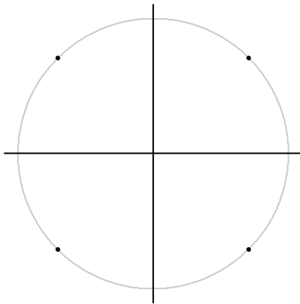
Fig. 4-18: Constellation diagram for DQPSK (INMARSAT and NATURAL) including the symbol mapping
