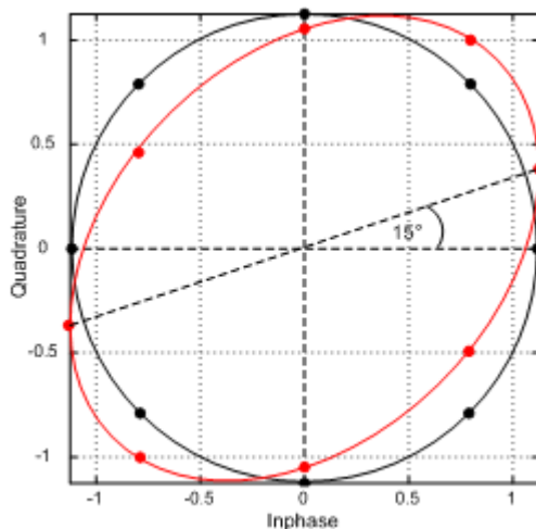
Fig. 4-55: Effect of Quadrature Error
