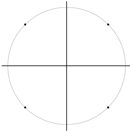
Fig. 4-27: MSK (for GSM and NATURAL) and DMSK Constellation Diagram including the symbol mapping
