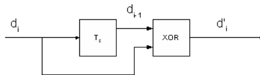
Fig. 4-28: DMSK: differential encoder in the transmitter
