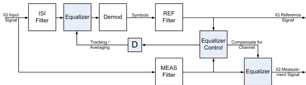
Fig. 4-48: An equalizer filter can be activated in the reference and measurement signal path. The filter coefficients are determined in such a way that the error vector magnitude (EVM) is minimized.
