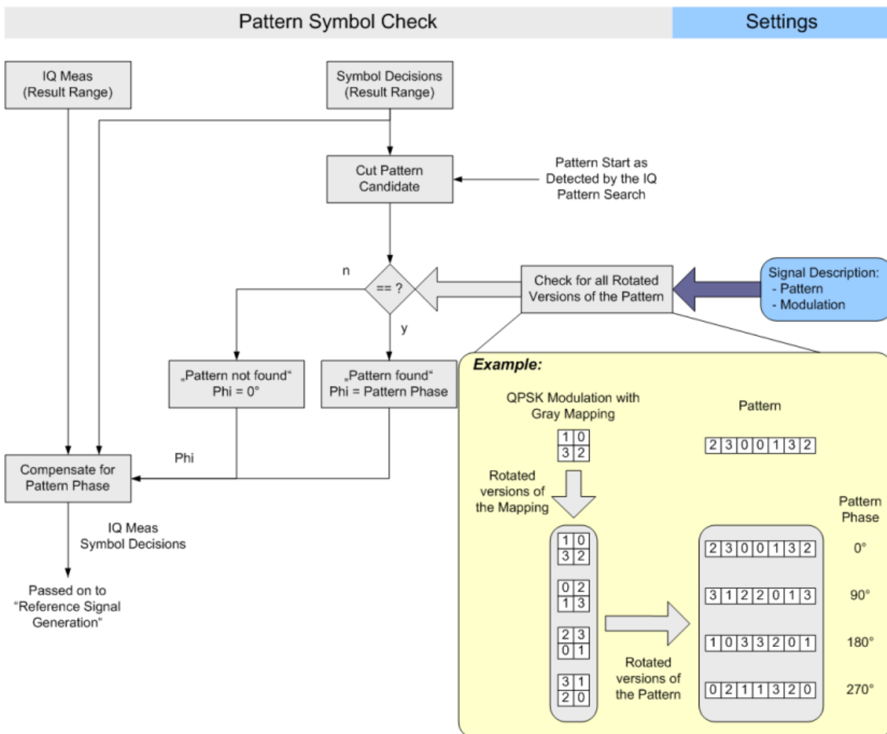
Fig. 4-45: Pattern Symbol Check algorithm
