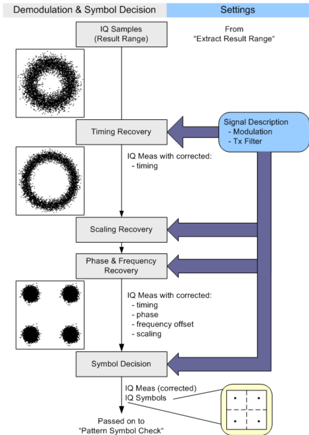
Fig. 4-44: Demodulation and Symbol Decision algorithm
