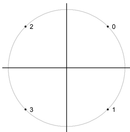
Fig. 4-16: Constellation diagram for 3\pi/4 QPSK including the symbol mapping for EDGE
