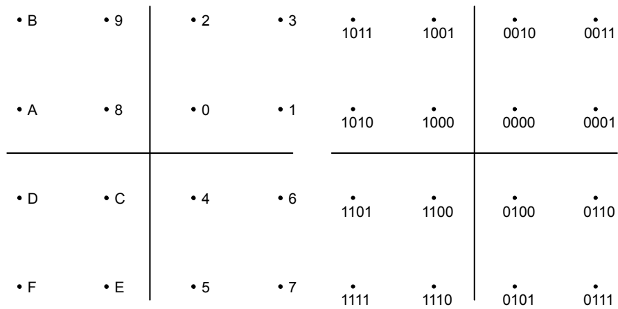
Fig. 4-31: Constellation diagram for 16QAM including the logical symbol mapping for DVB-C (hexadecimal and binary)
