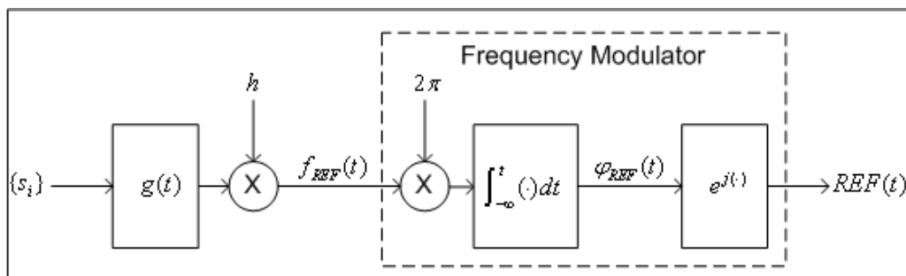
Fig. 4-58: Reference complex baseband FSK signal generation
