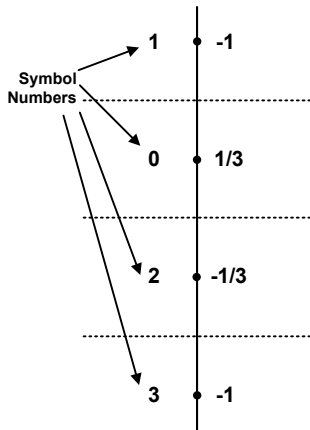
Fig. 4-25: Constellation diagram for 4FSK for APCO C4FM and APCO Phase 2 including the logical symbol mapping
