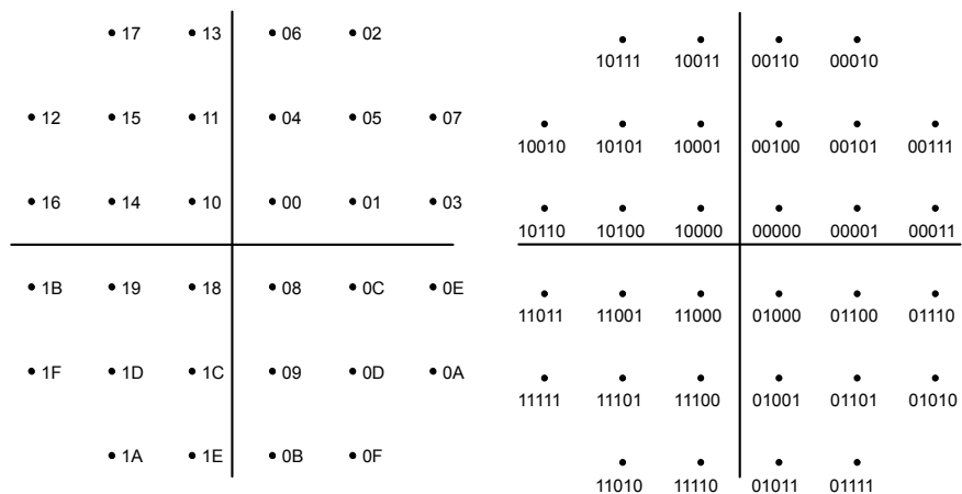
Fig. 4-32: Constellation diagram for 32QAM including the logical symbol mapping for DVB-C (hexadecimal and binary)
