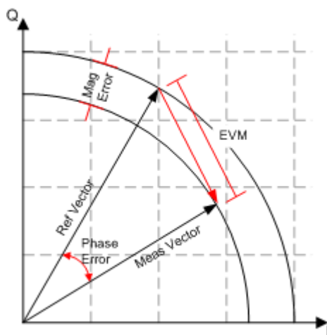
Fig. 4-51: Modulation error: EVM, magnitude error, phase error
