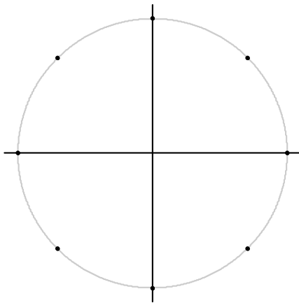
Fig. 4-19: Constellation diagram for D8PSK including the symbol mapping for APCO25, APCO25 Phase 2, GRAY, NATURAL and TETRA
