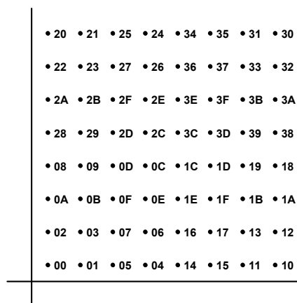
Fig. 4-35: Constellation diagram for 256QAM including the logical symbol mapping (hexadecimal); the figure shows the upper right section of the diagram only
