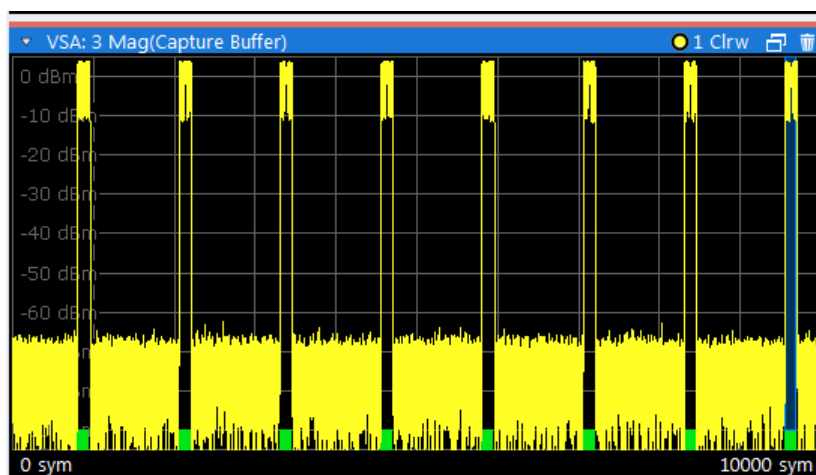
Fig. 4-63: Result ranges for a burst signal
