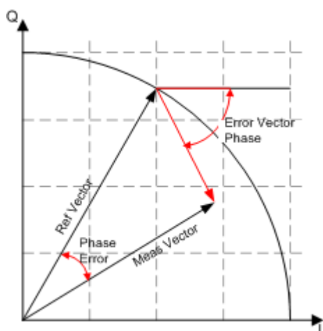
Fig. 4-52: Modulation error: Phase error, error vector phase
