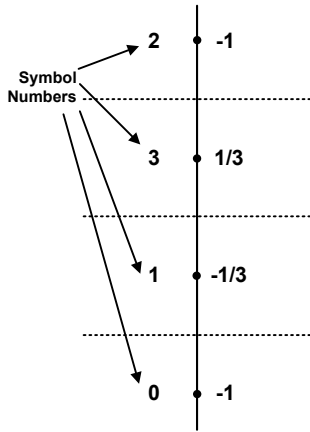
Fig. 4-24: Constellation diagram for 4FSK (GRAY) including the logical symbol mapping
