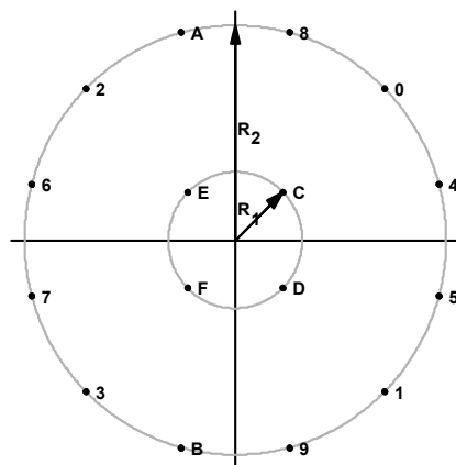
Fig. 4-40: Constellation diagram for 16APSK including the logical symbol mapping for DVB-S2
