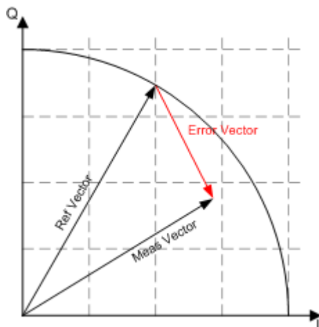
Fig. 4-50: Modulation error: error vector
