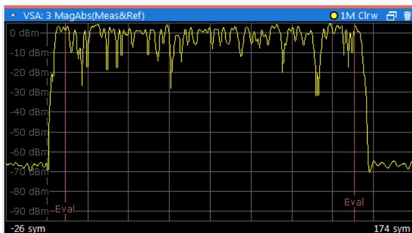
Fig. 4-65: Evaluation lines in absolute magnitude diagram
