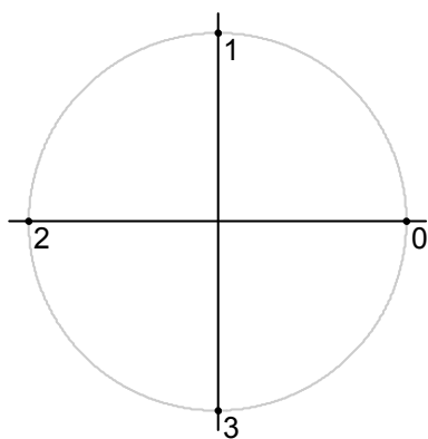
Fig. 4-17: Constellation diagram for \pi/4 QPSK (Natural) including the symbol mapping
