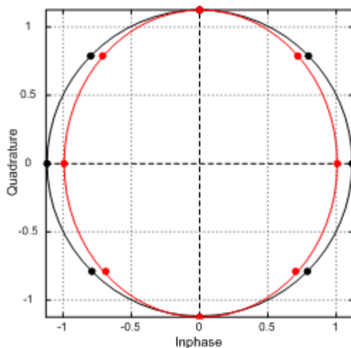
Fig. 4-54: Effect of gain imbalance
