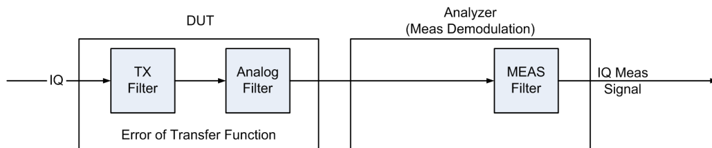
Fig. 4-46: General processing in the modulation- and demodulation stages
