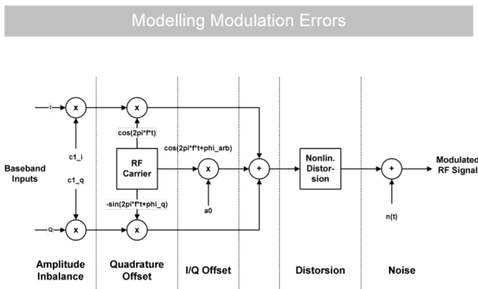
Fig. 4-49: Modelling Modulation Errors
