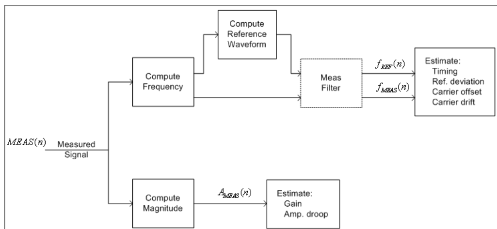
Fig. 4-59: FSK Estimation Strategy
