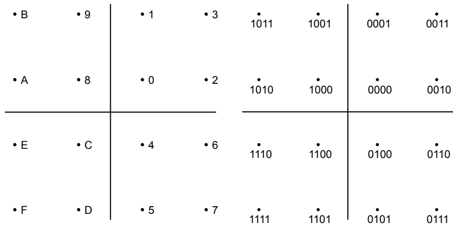
Fig. 4-30: Constellation diagram for 16QAM including the logical symbol mapping for EDGE (hexadecimal and binary)
