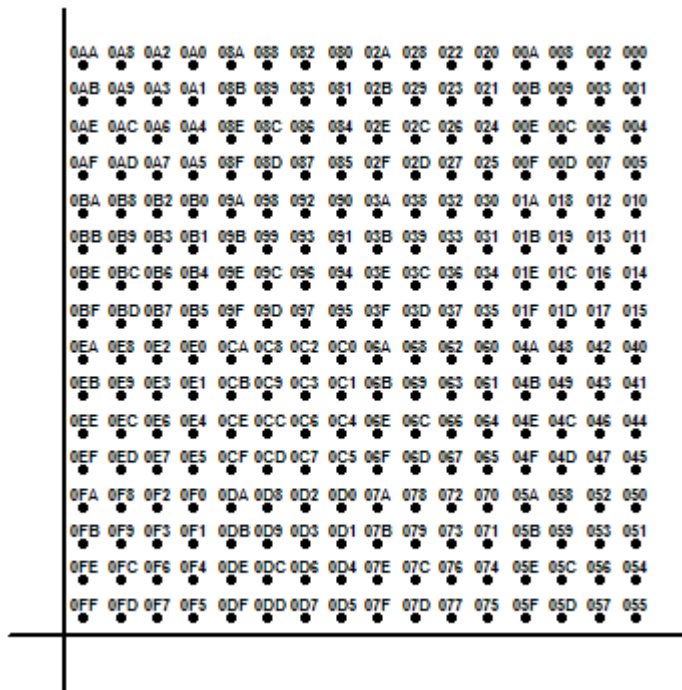
Fig. 4-37: Constellation diagram for 1024QAM including the logical symbol mapping (hexadecimal); the figure shows the upper right section of the diagram only
